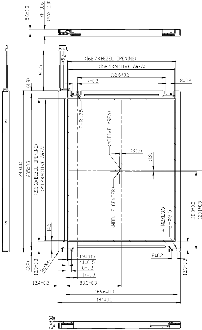
Fig.1 LCM outline dimensions
